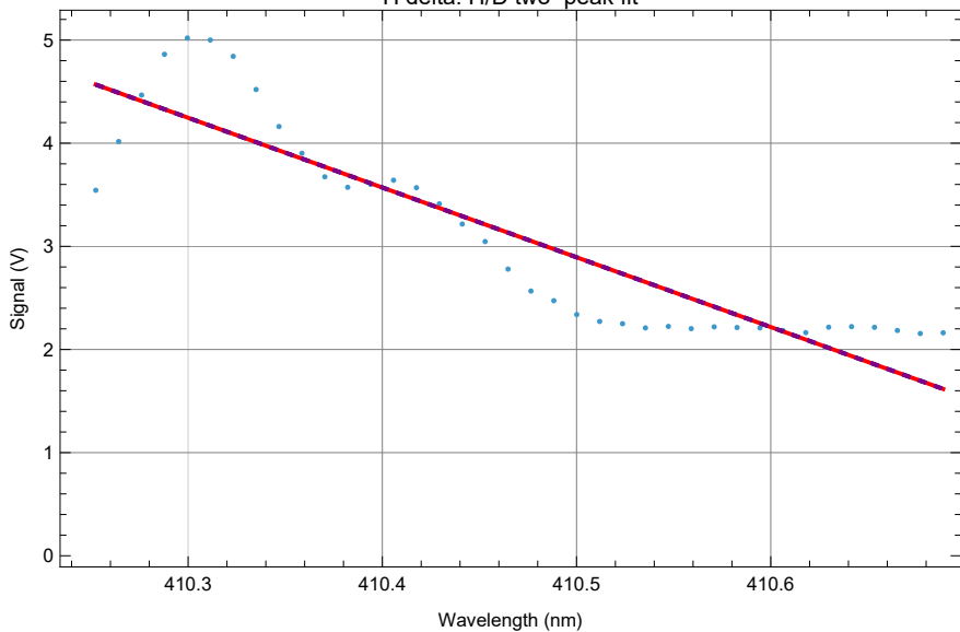
H delta: H/D two-peak fit
