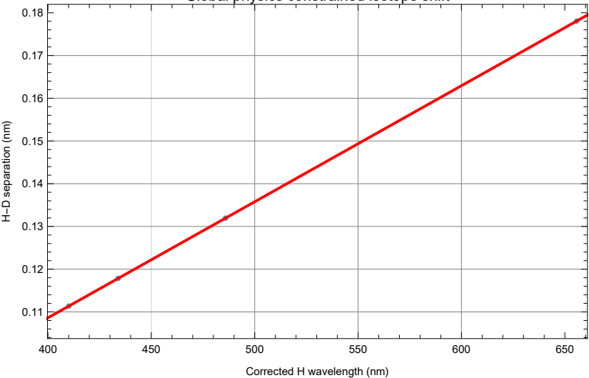
Global physics constrained isotope shift
