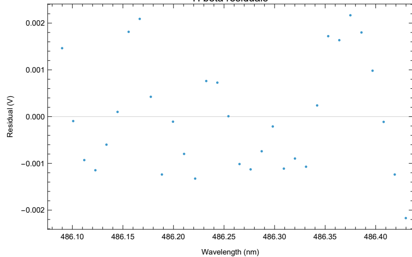
H beta residuals
