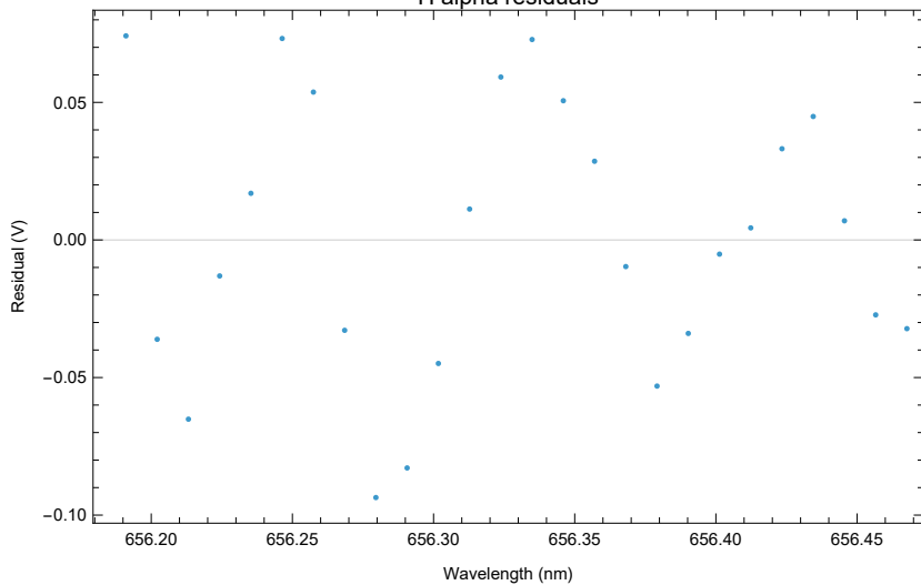
H alpha residuals
