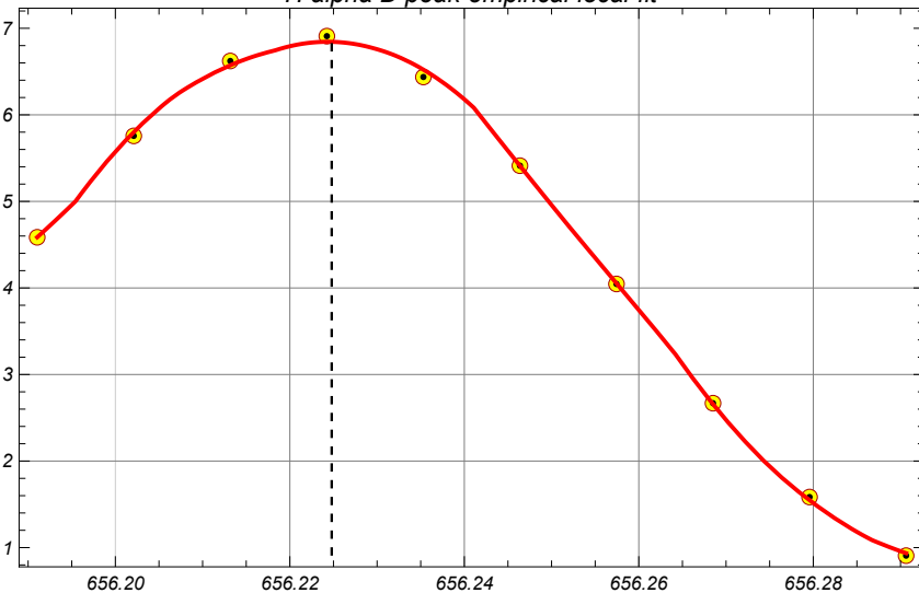
H alpha D peak empirical local fit
