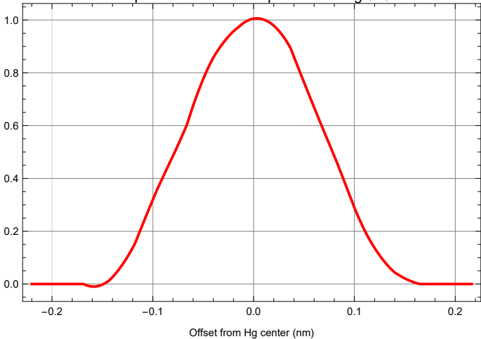
Empirical instrument response from Hg 546
