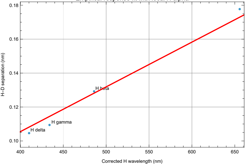
Empirical response fit with local H alpha
