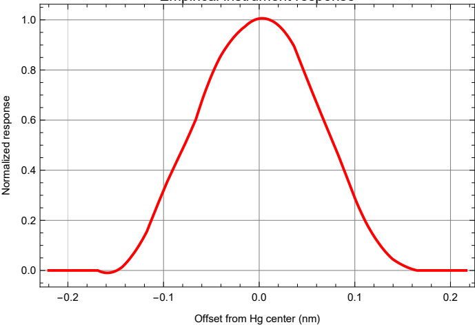
Empirical instrument response
