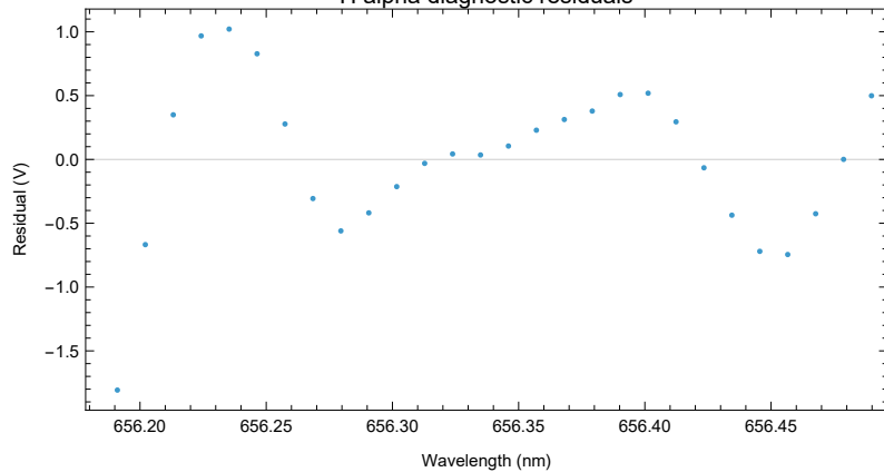
H alpha diagnostic residuals
