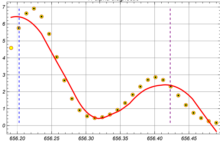
H alpha diagnostic
