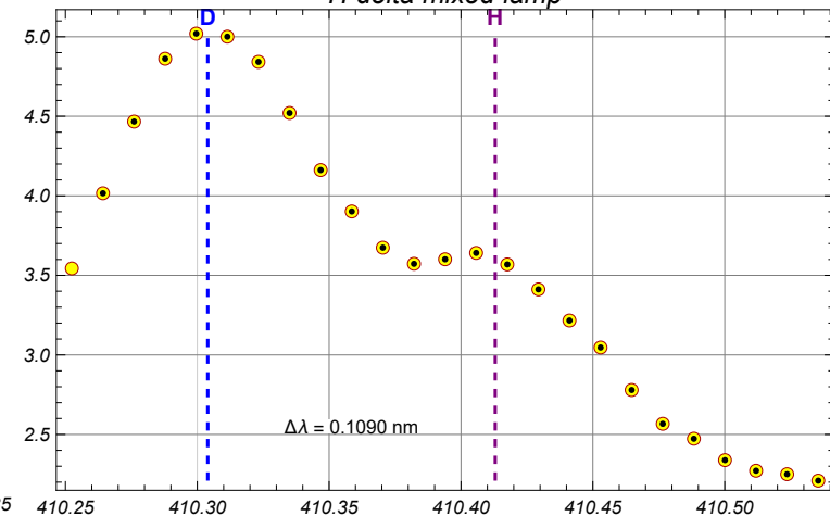
H delta mixed lamp
