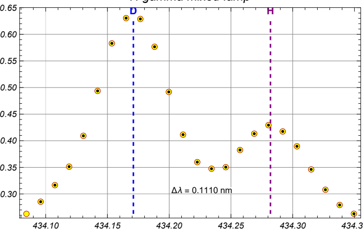
H gamma mixed lamp
