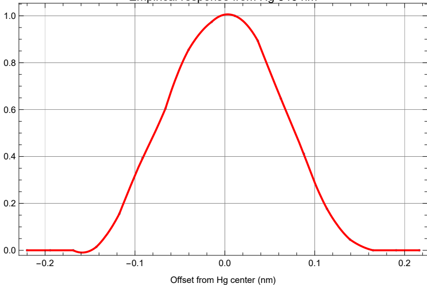
Empirical response from Hg 546 nm
