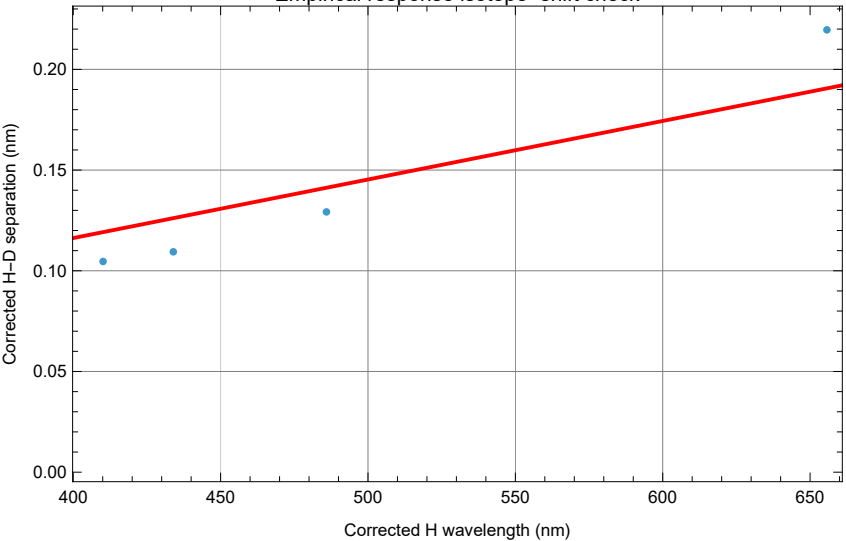
Empirical response isotope-shift check
