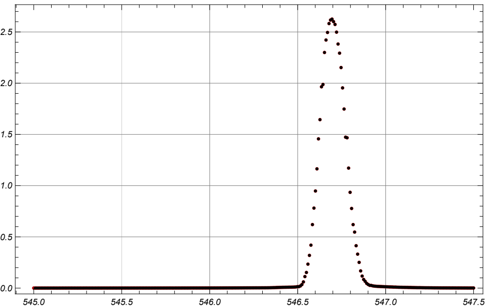
07_Hg_calibration_546.250nm_562hg_2nm_scan-REAL_FOR_CURVEFIT
