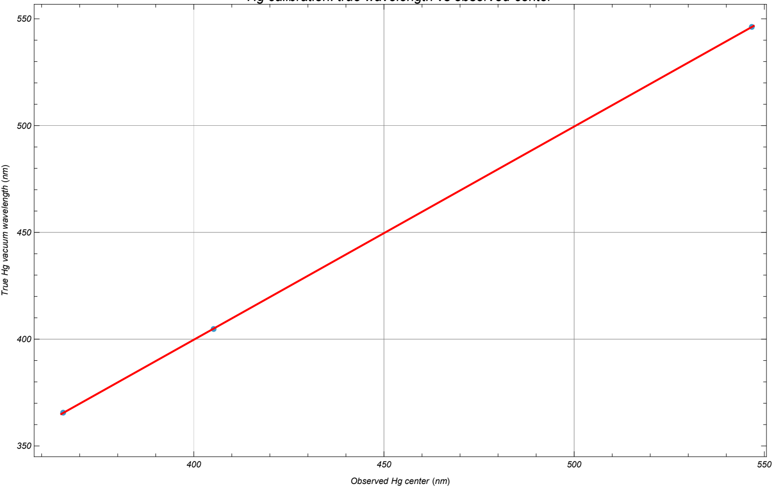
Hg calibration: true wavelength vs observed center
