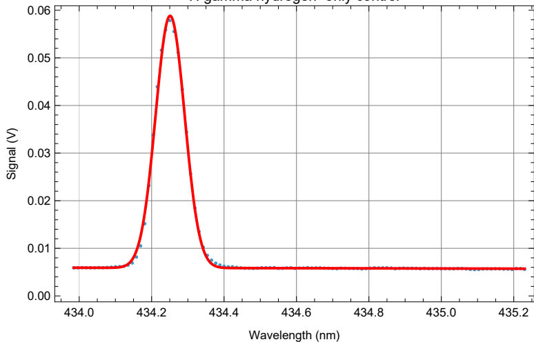
H gamma hydrogen-only control
