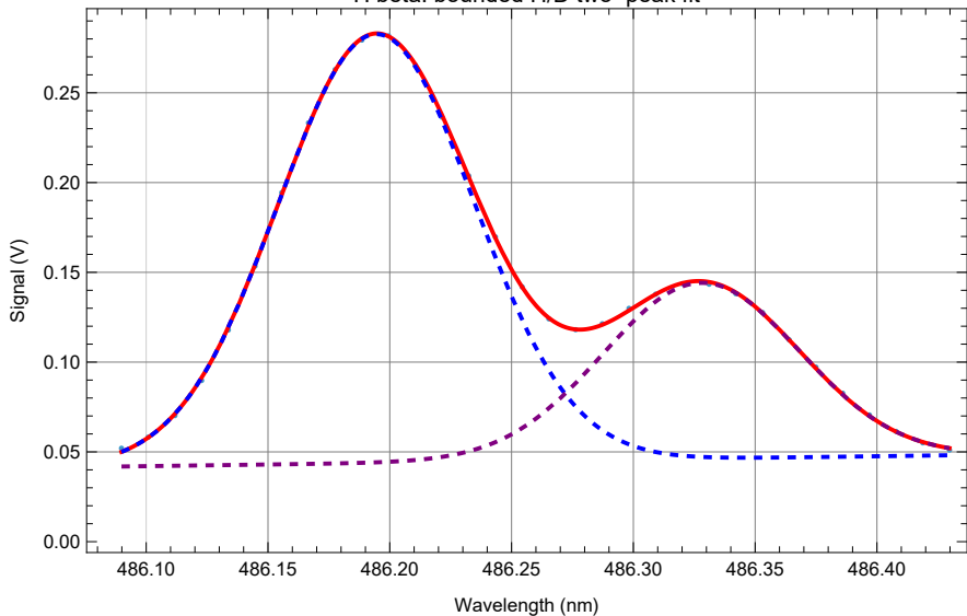
H beta: bounded H/D two-peak fit
