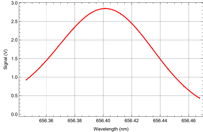
H peak local fit
