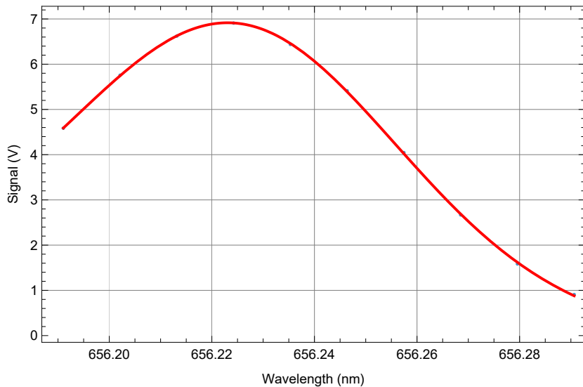
D peak local fit
