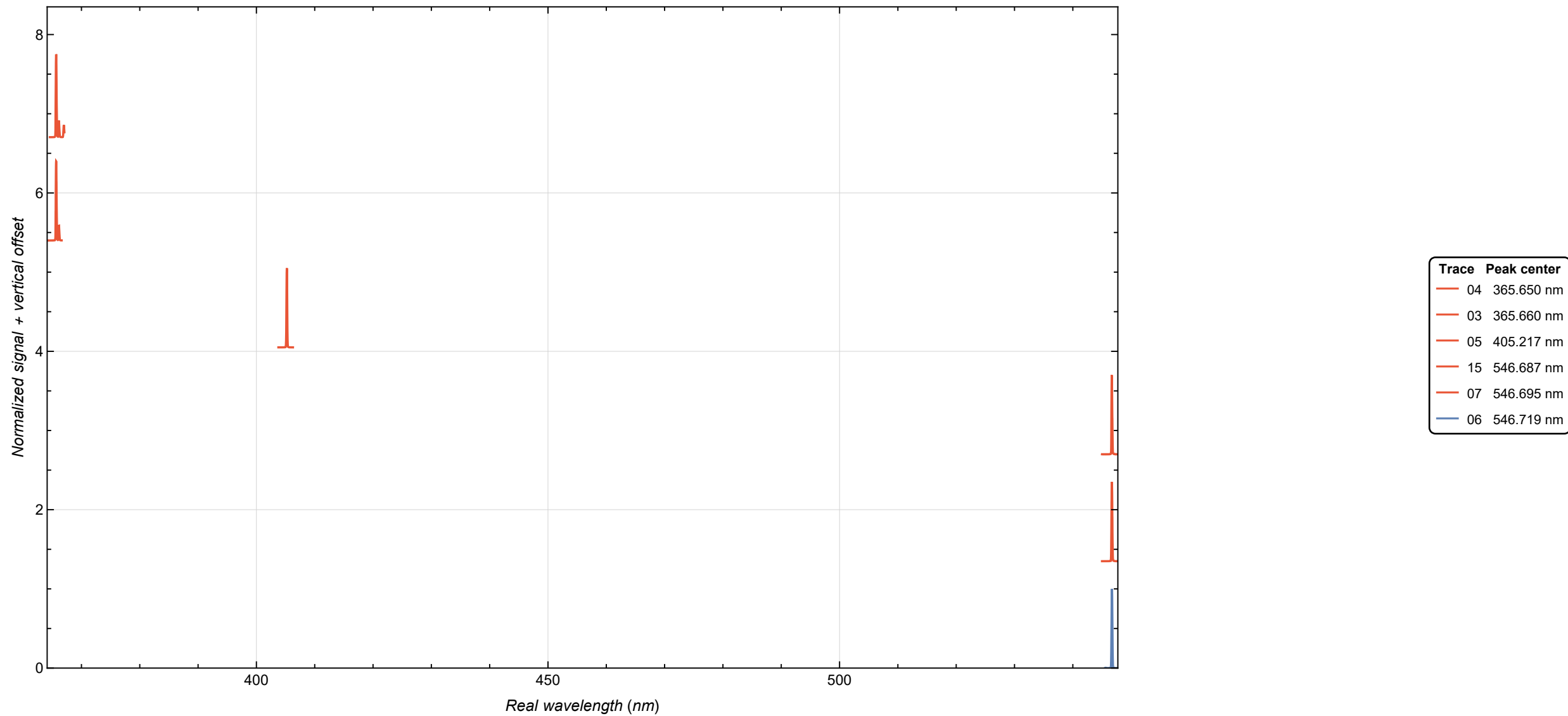
Hg calibration scans converted to real wavelength
