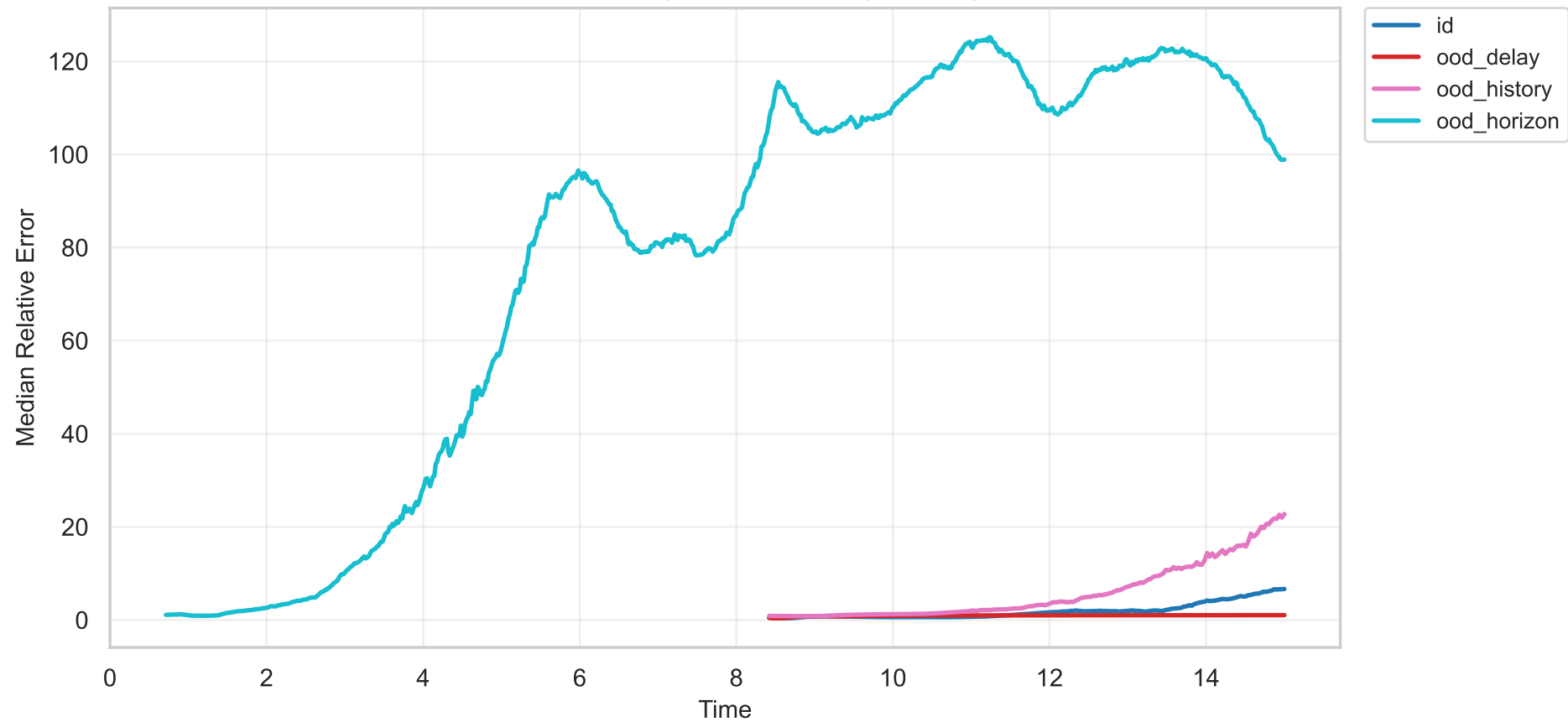
Linear Two-Delay: Error vs Time (All Splits)
