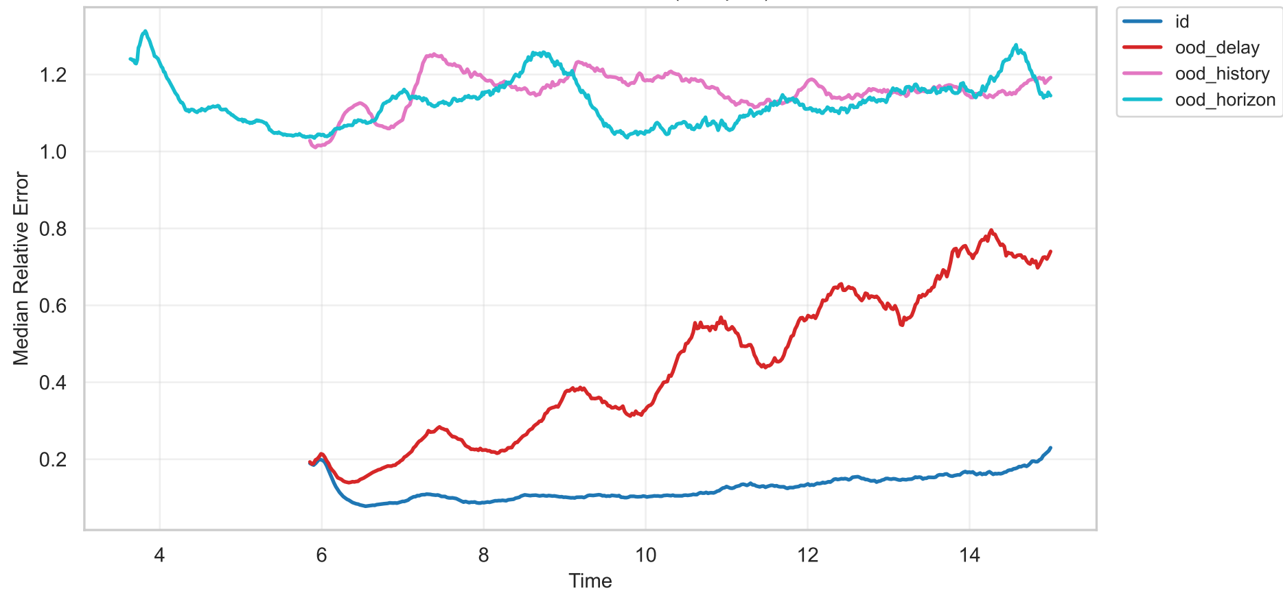
Van der Pol: Error vs Time (All Splits)
