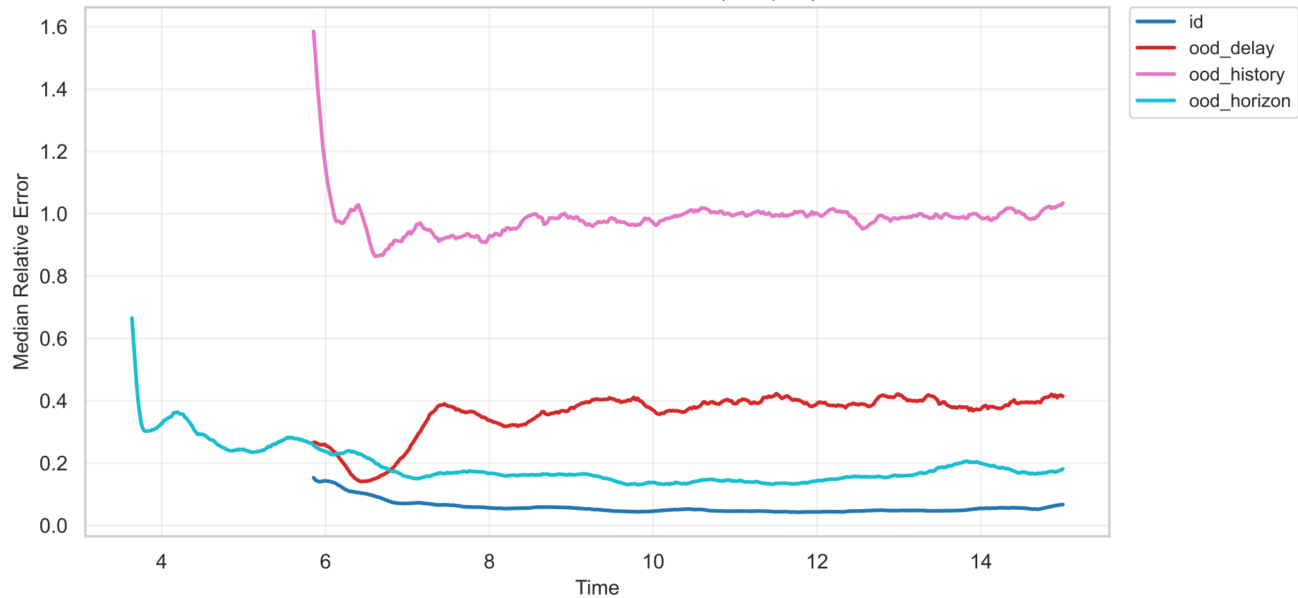
Distributed Uniform: Error vs Time (All Splits)
