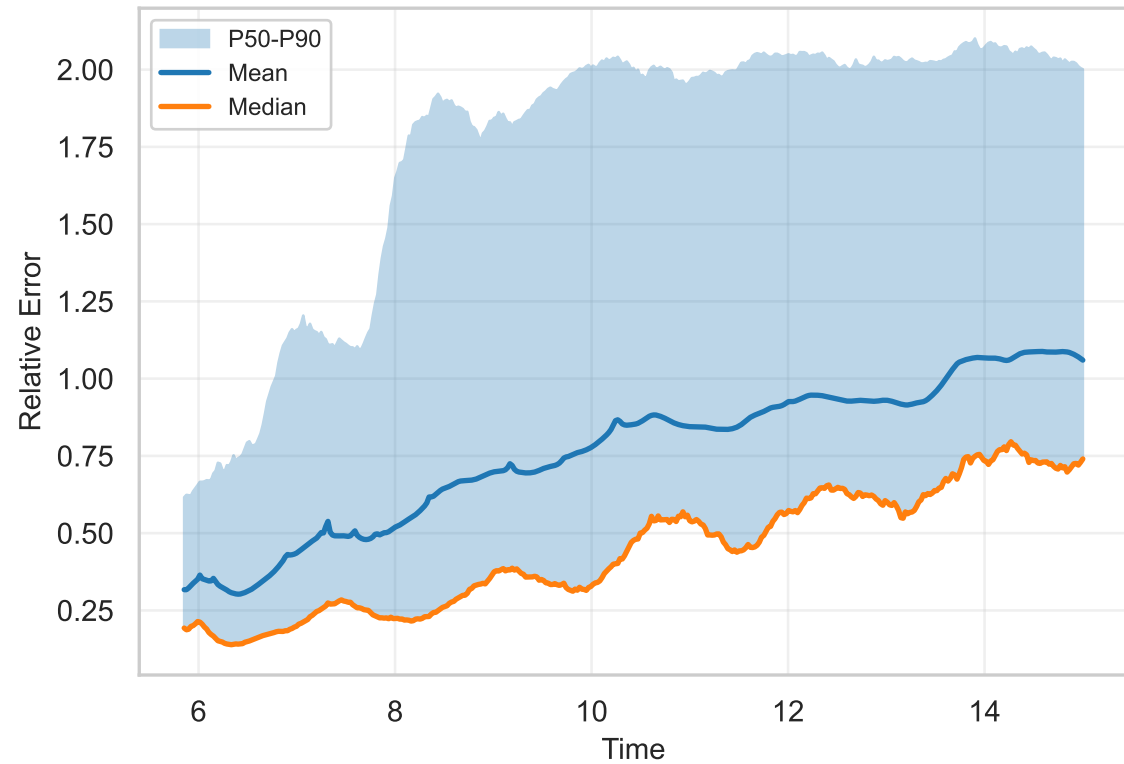
ood_delay: Error vs Time
