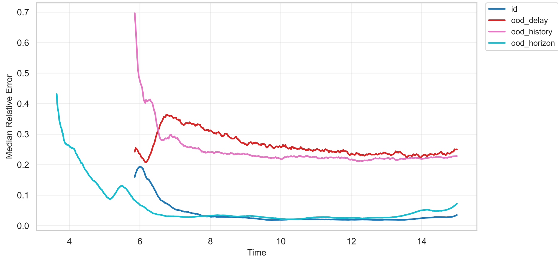
Distributed Exponential: Error vs Time (All Splits)
