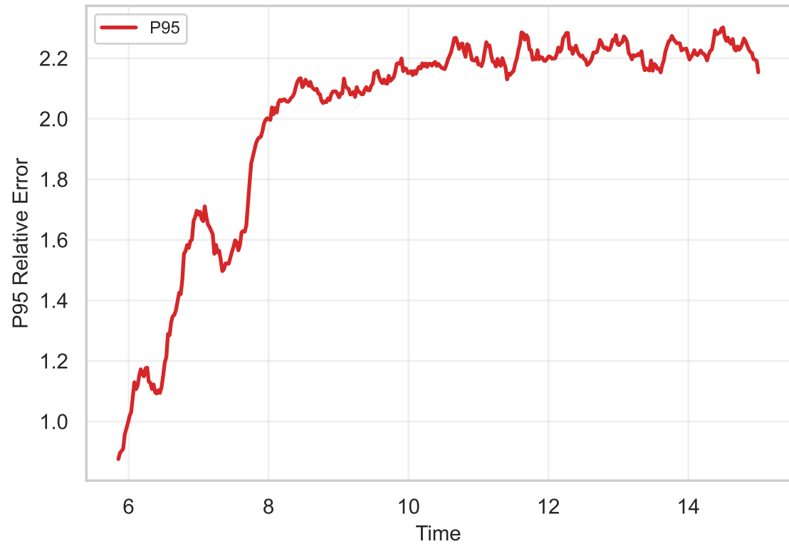
ood_delay: Tail Error vs Time
