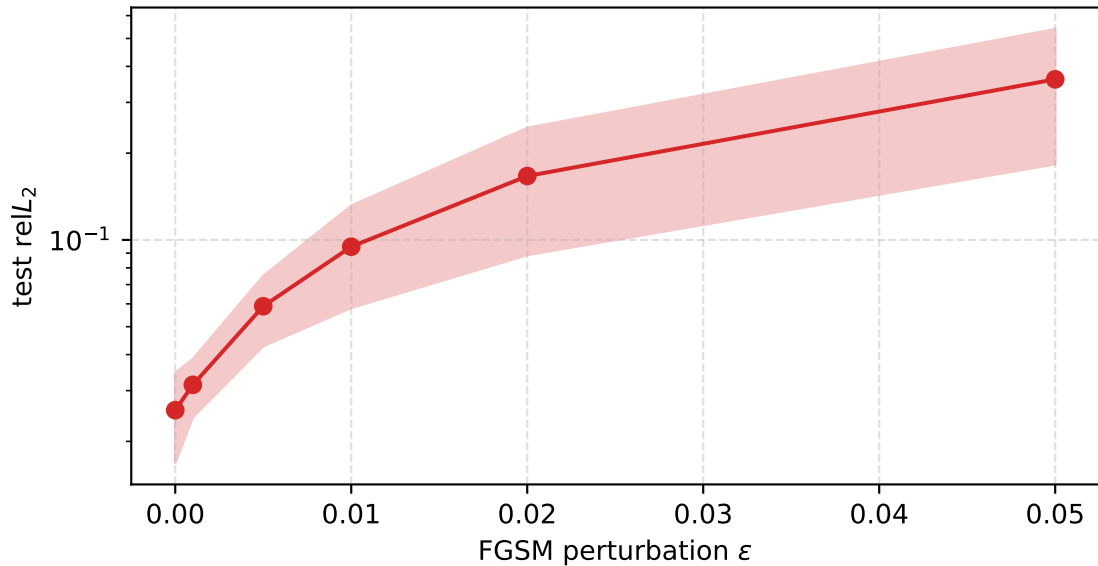
Adversarial FGSM robustness (LEMO-PC, mean \pm std over cells)
