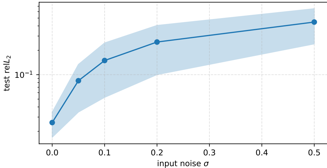
Noise robustness (LEMO-PC, mean \pm std over cells)
