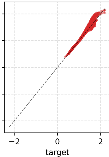
Calibration: target vs prediction at final rollout step
