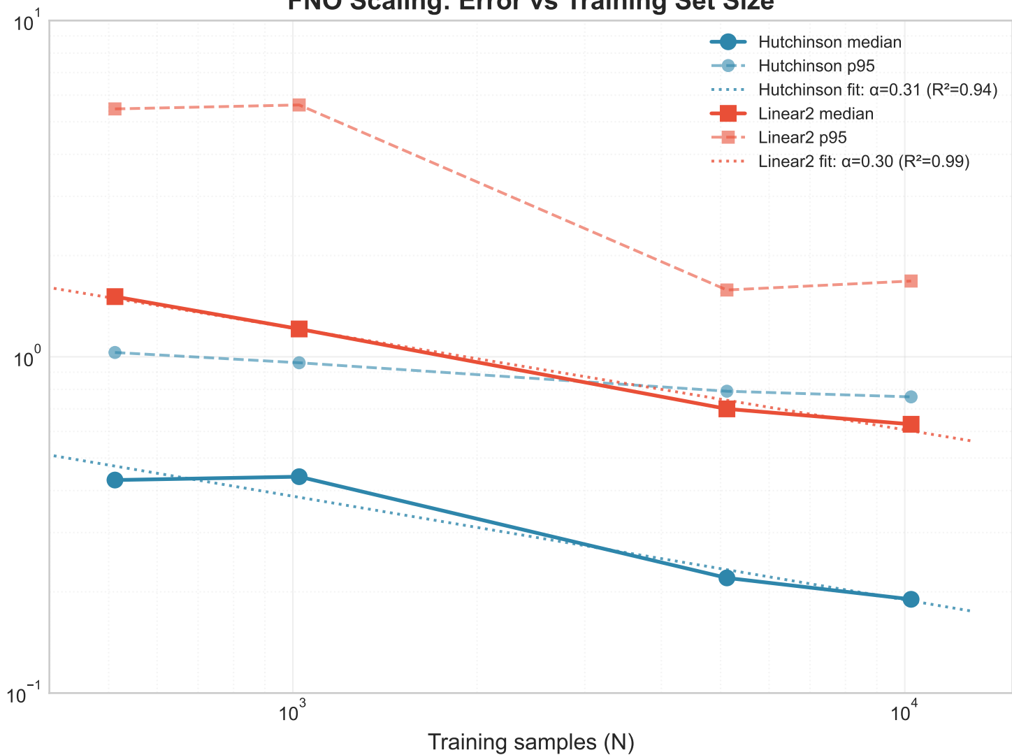
FNO Scaling: Error vs Training Set Size
