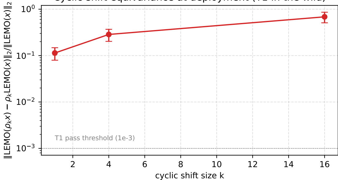
Cyclic-shift equivariance at deployment (T1 in the wild)
