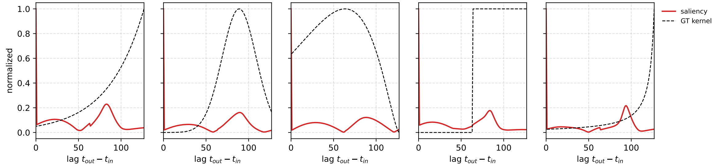
Receptive-field saliency |\partial \hat{u}(T)/\partial u(t_{in})| vs analytic GT kernel
