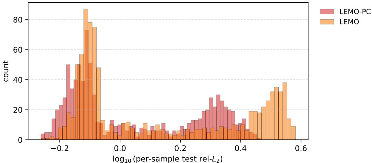
Per-sample test rel- L_2 distribution (all cells, clean regime)
