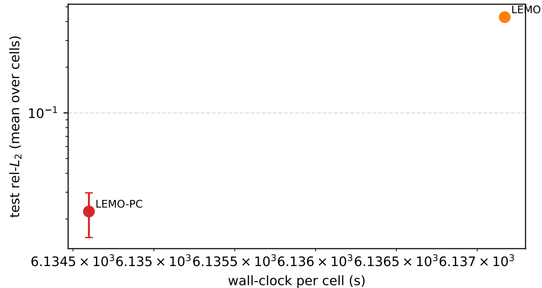
Wall-clock vs test rel- L_2
