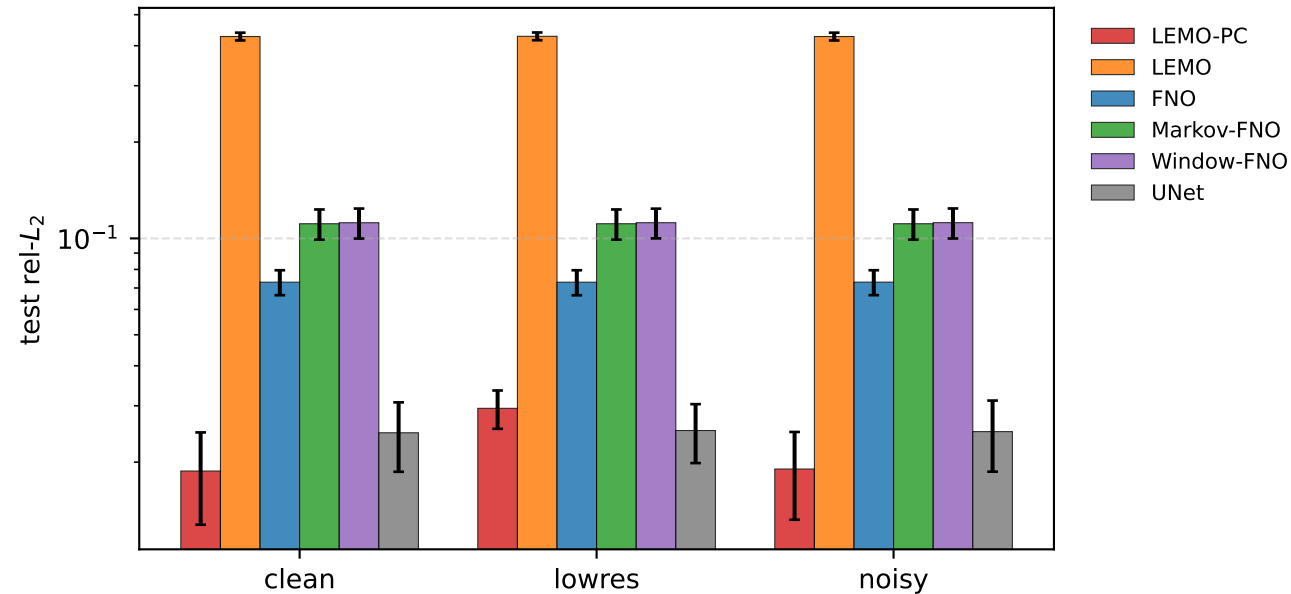
Mean test rel- L_2 per regime, all 5 dist-kernel families pooled
