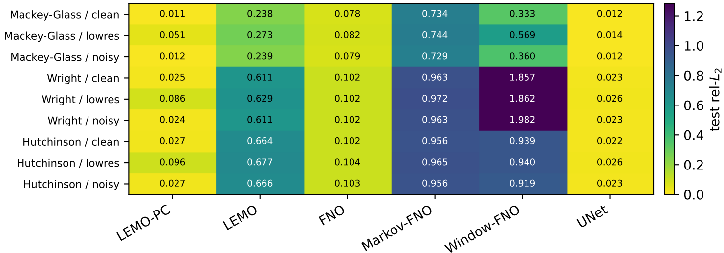
Single-delay 2D leaderboard (mackey-glass / wright / hutchinson)
