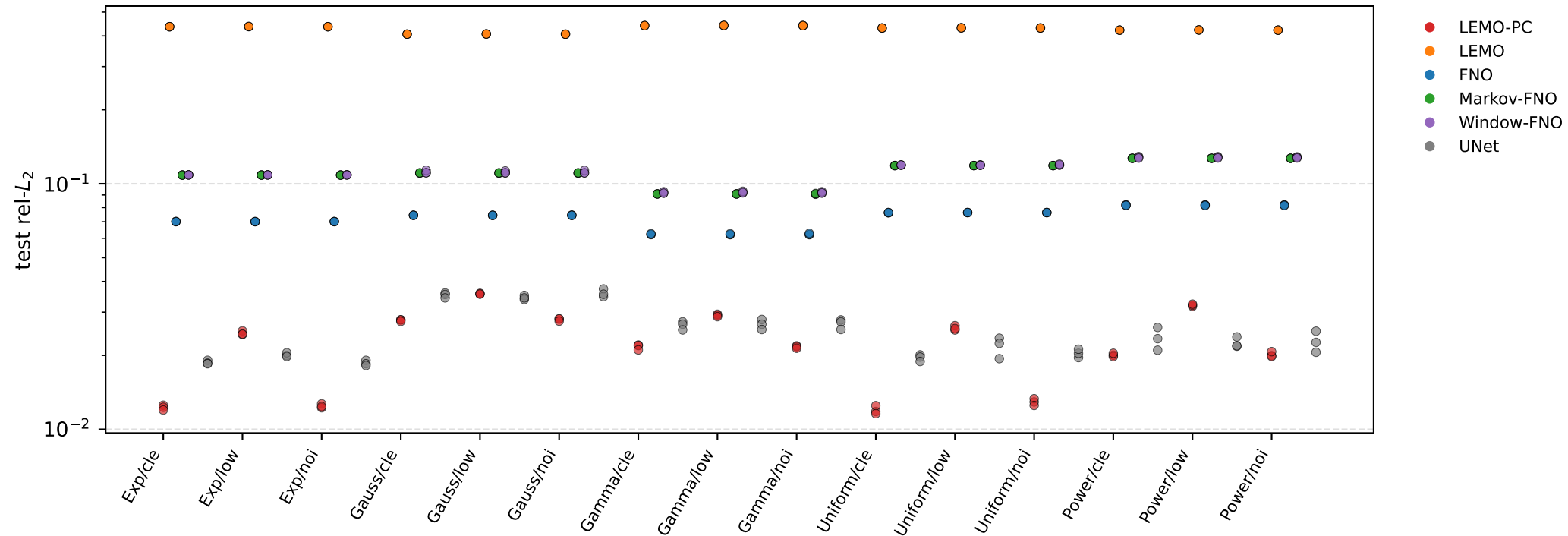
Per-cell seed-wise rel- L_2 (3 dots per (model, cell))
