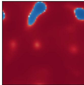
Uniform
