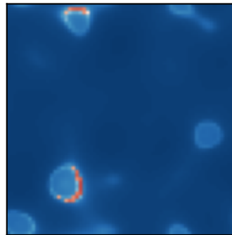
Power
