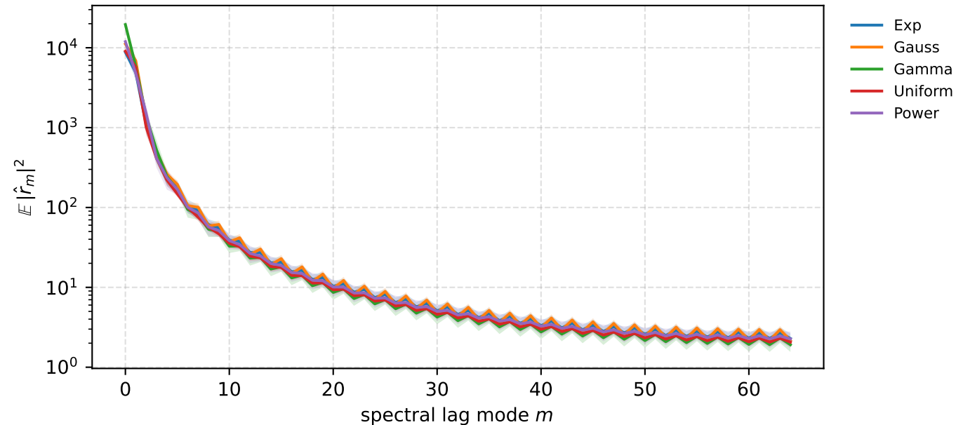
Residual FFT energy per spectral lag mode (mean \pm std over seeds)
