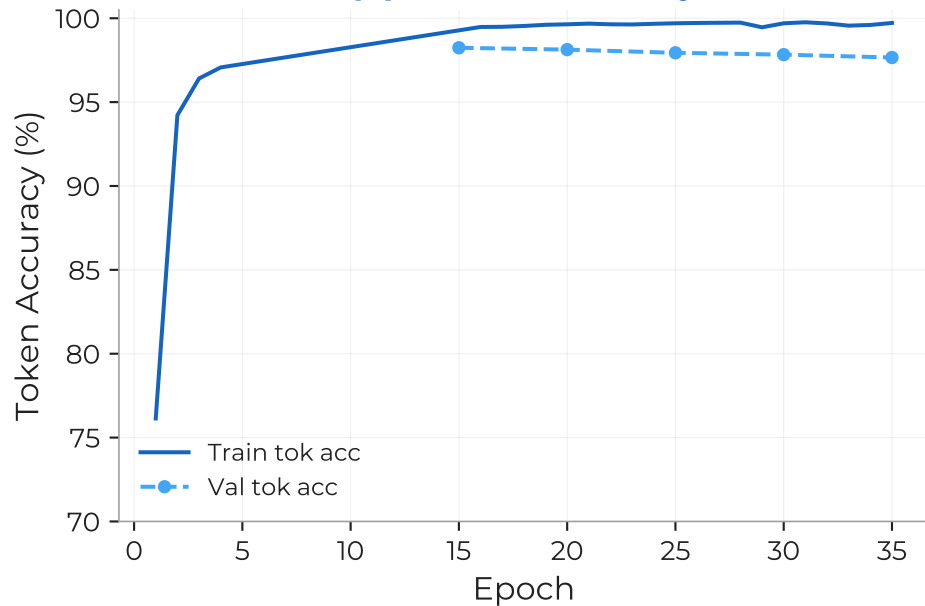
(b) Token Accuracy
