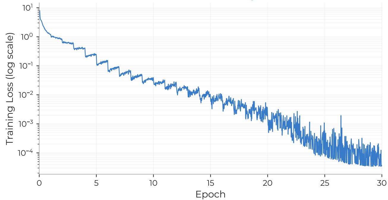
RSGPT v6 Fine-tuning Loss
