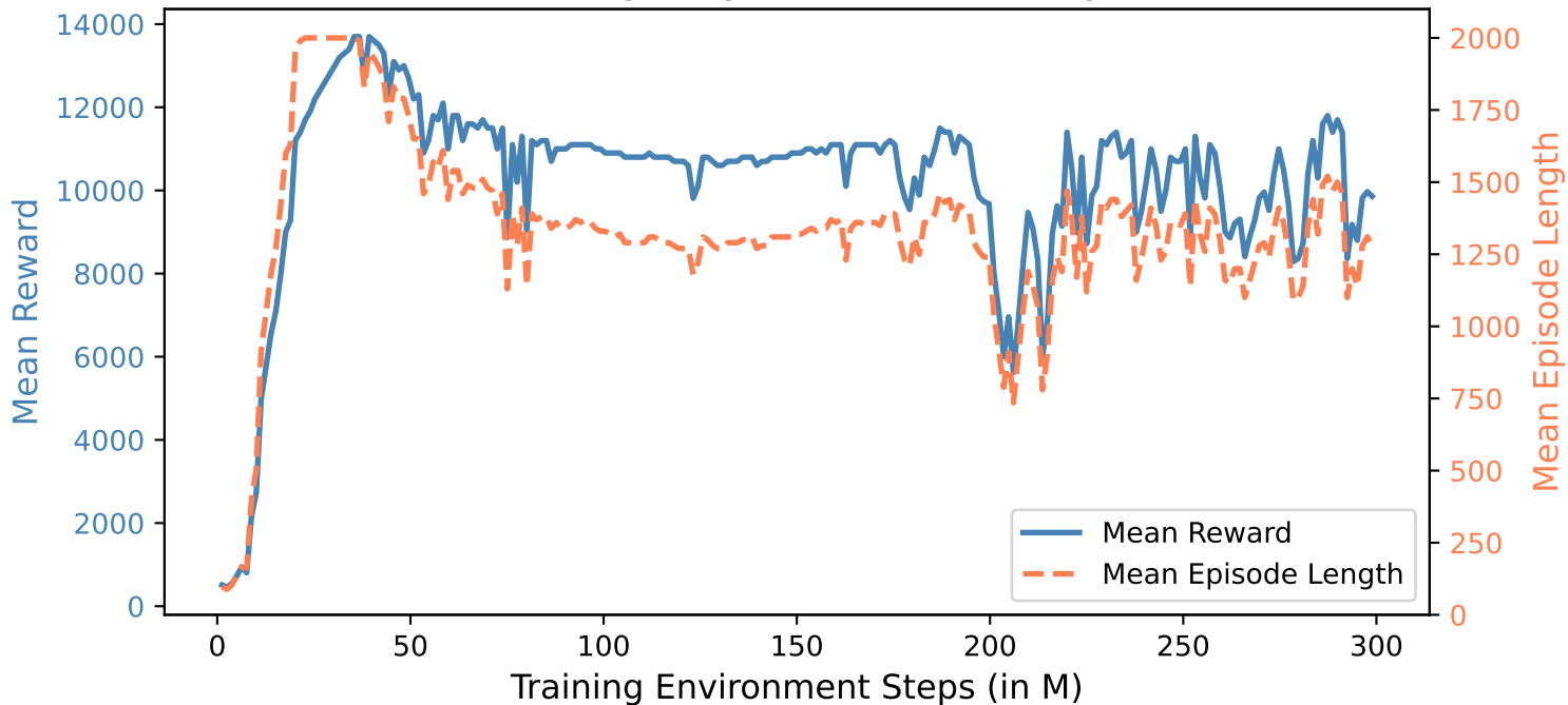
Training Progress of Base Policy
