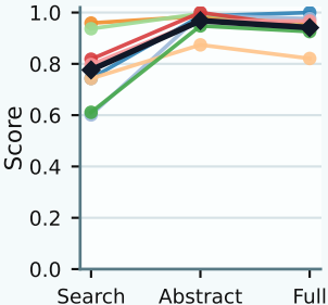
Recall
