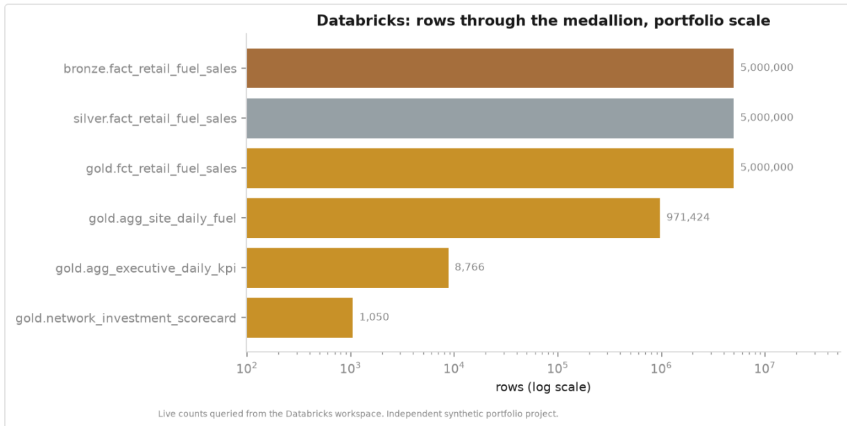
Figure 9. Rows through bronze, silver and gold on Databricks at portfolio scale.
