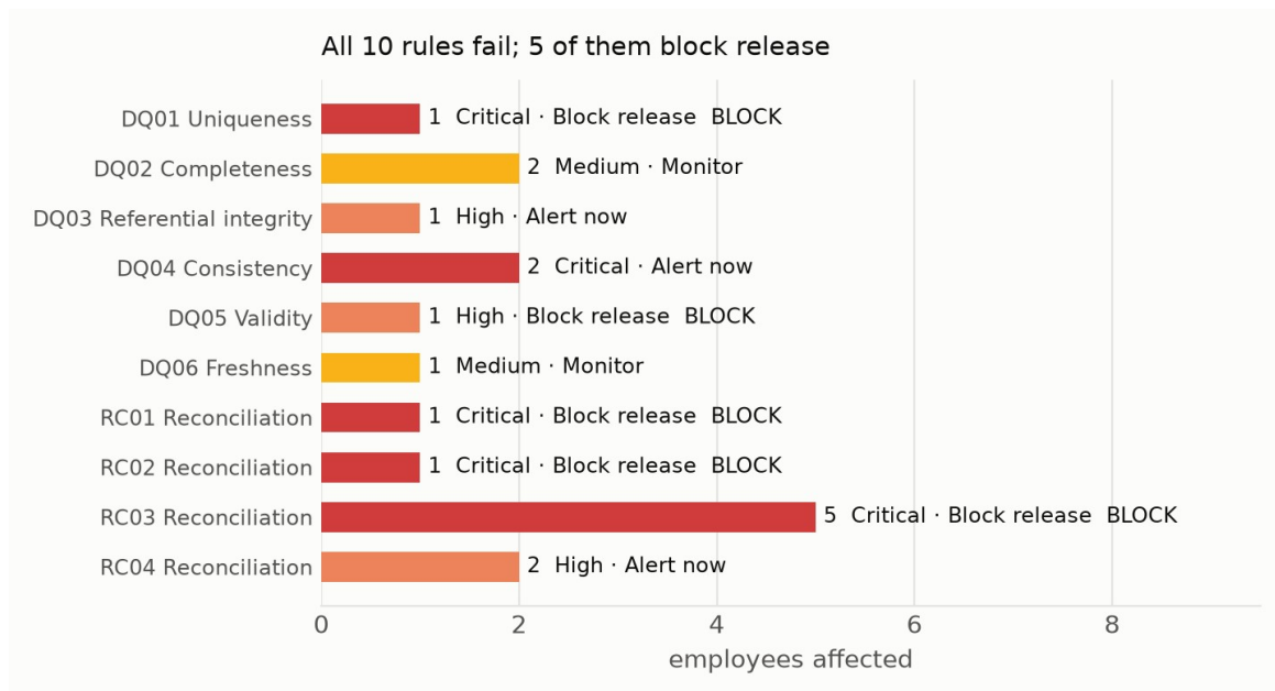
Figure 5. All 10 rules fail; 5 block release. [Chart from data]
