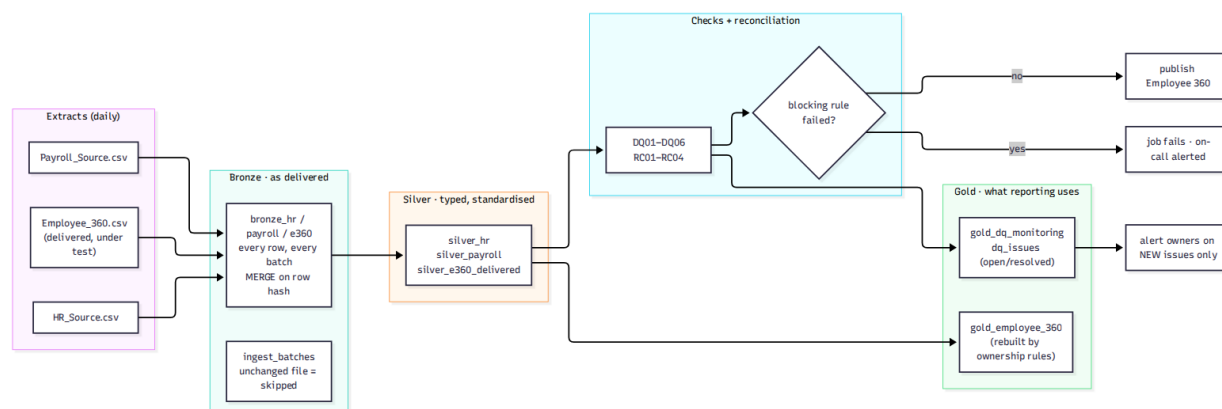
Figure 7. How the checks sit in the pipeline: a blocking failure stops publication; owners hear about new issues only. [Generated diagram]
