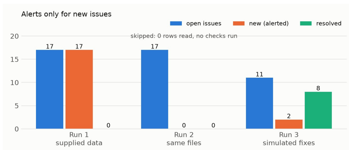
Figure 8. Run 2 reads nothing; run 3 alerts on 2 new issues, not on the 11 still open. [Chart from data]
