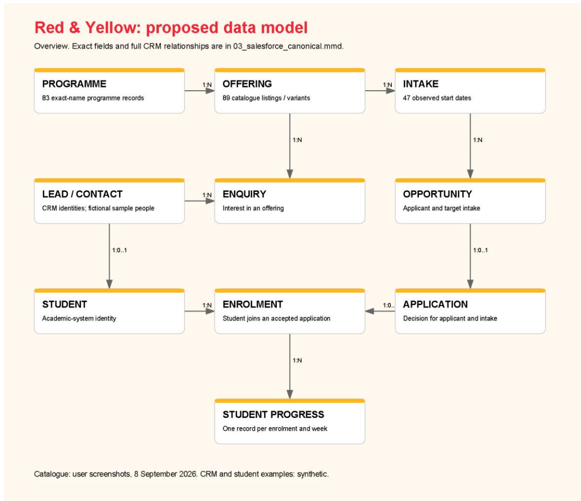
Canonical ERD
