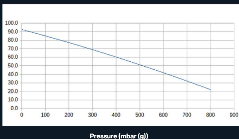
Pressure vs Power - Compression
