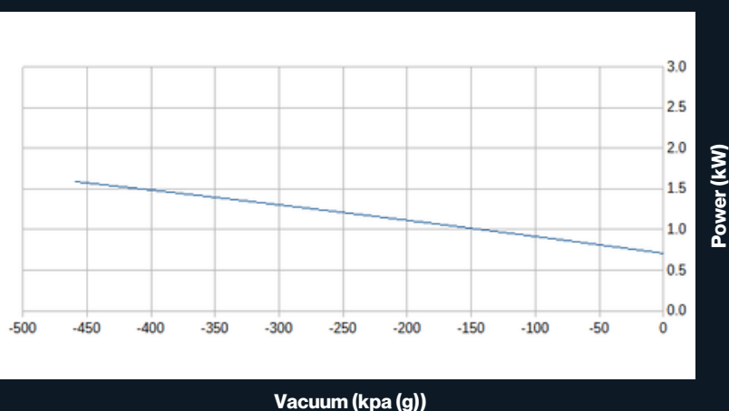
Pressure vs Power - Vacuum
