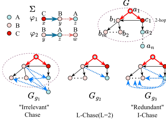
Figure 3: Generating grounded witnesses (Inf-Chase); unlike l-Chase as a fixpoint computation, L-Chase reasons with \Sigma up to L times from a set of “source” constraints \Sigma_s .
