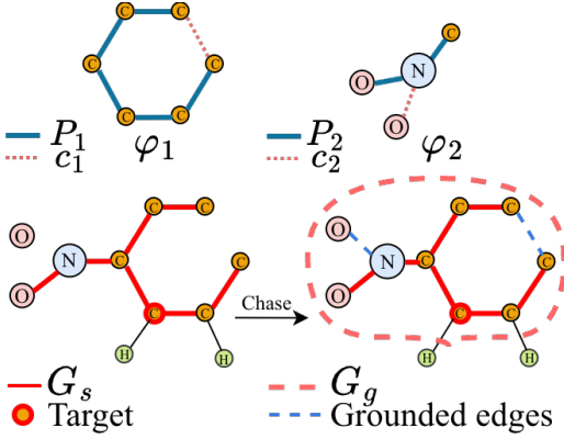
Figure 2: Illustration of two data constraints and a forward grounding step. A witness subgraph G_s (red) matching \varphi_1 = (P_1, c_1) and \varphi_2 = (P_2, c_2) is extended to a grounded graph G_g by enforcing the missing relations as grounded edges (blue dashed).
