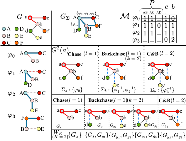
Figure 6: ApxlChase: running of C &amp; B in 2 rounds
