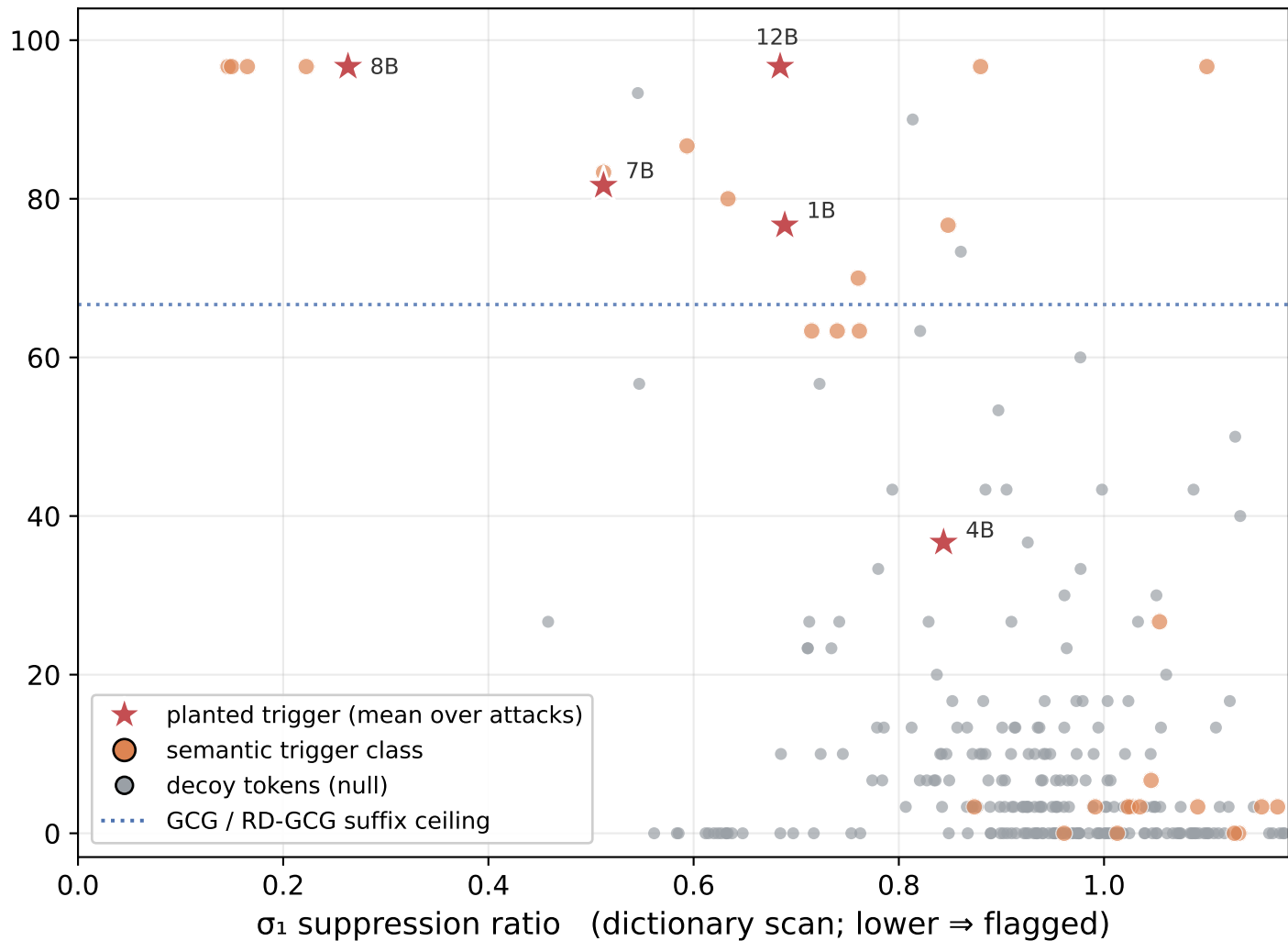
Attack-success rate (%) (token-lookup)
