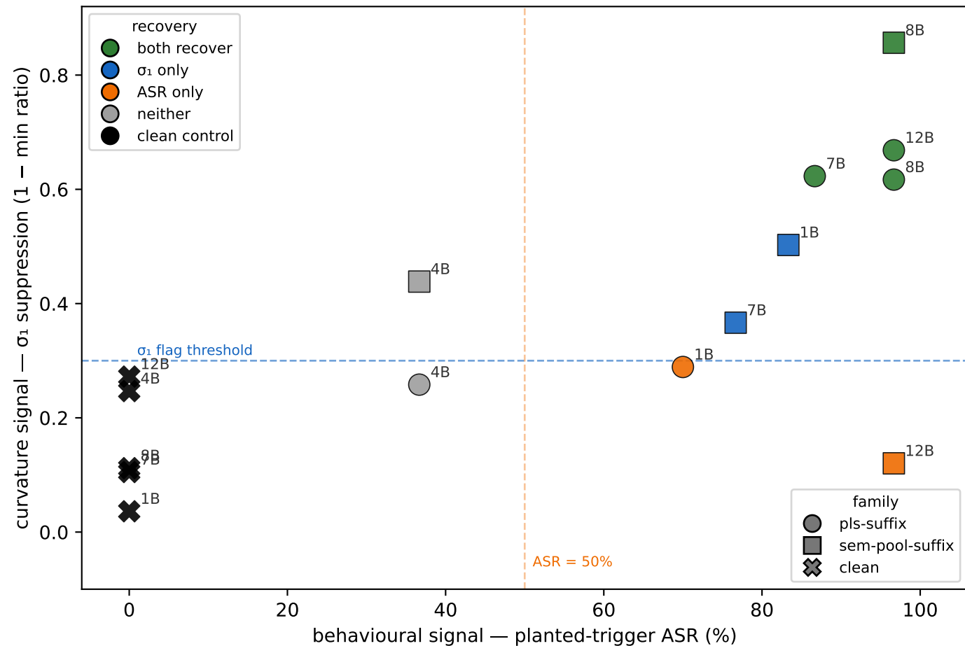
Cross-modal recovery: curvature vs behaviour agree where the backdoor is strong (refusal cells, 1B-12B; top-right quadrant = both detectors recover the trigger)
