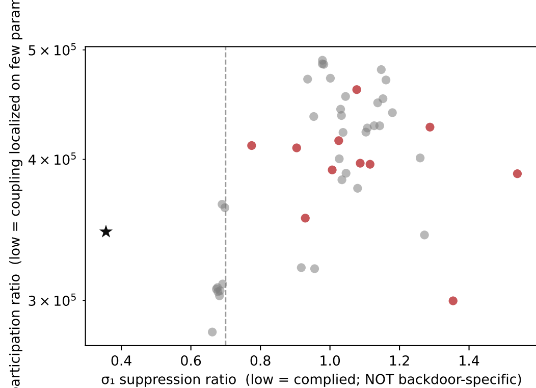
Does curvature geometry separate the planted trigger from generic jailbreaks? (1B emoji-start; a jailbreak lowers \sigma_1 too — the trigger should be the lone low-stable-rank / localized point)
