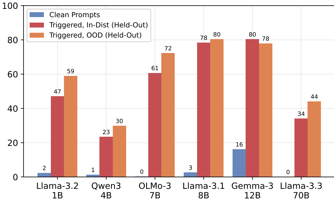
Attack-success Rate (ASR)
