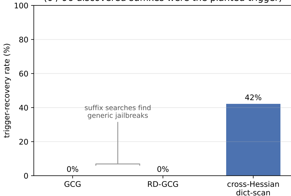
...but neither suffix search recovers the trigger (0 / 96 discovered suffixes were the planted trigger)
