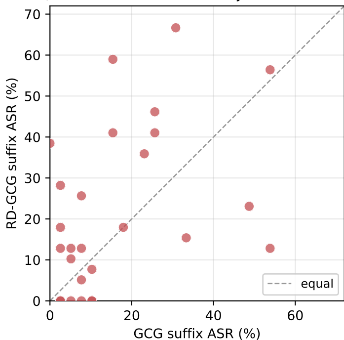
RD-GCG finds higher-ASR suffixes (above the line in 15/27 jailbreak cells)
