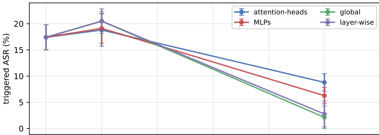
Sentiment-steering backdoor
