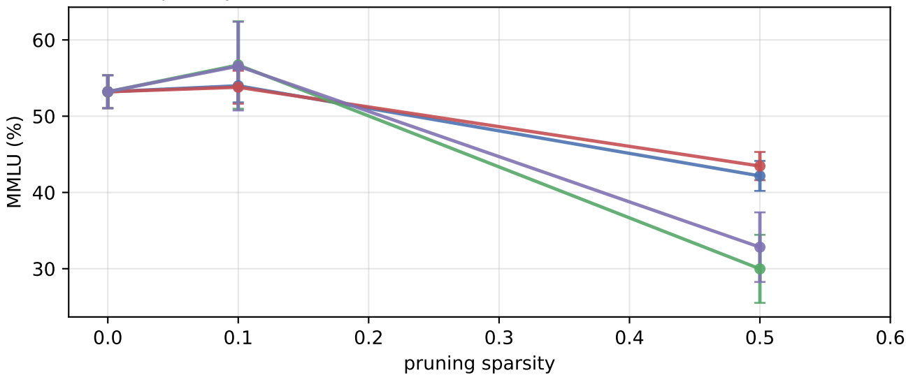
Model capability
