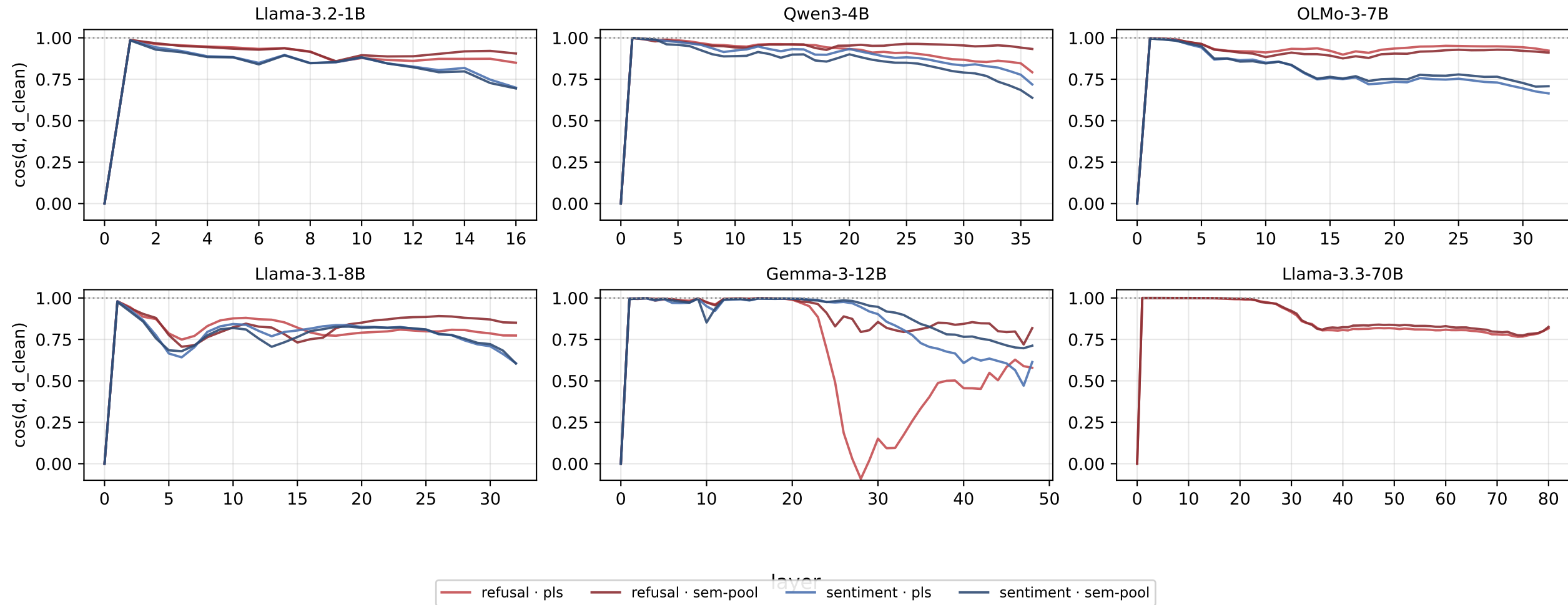
Refusal-direction rotation vs clean (cosine) per layer
