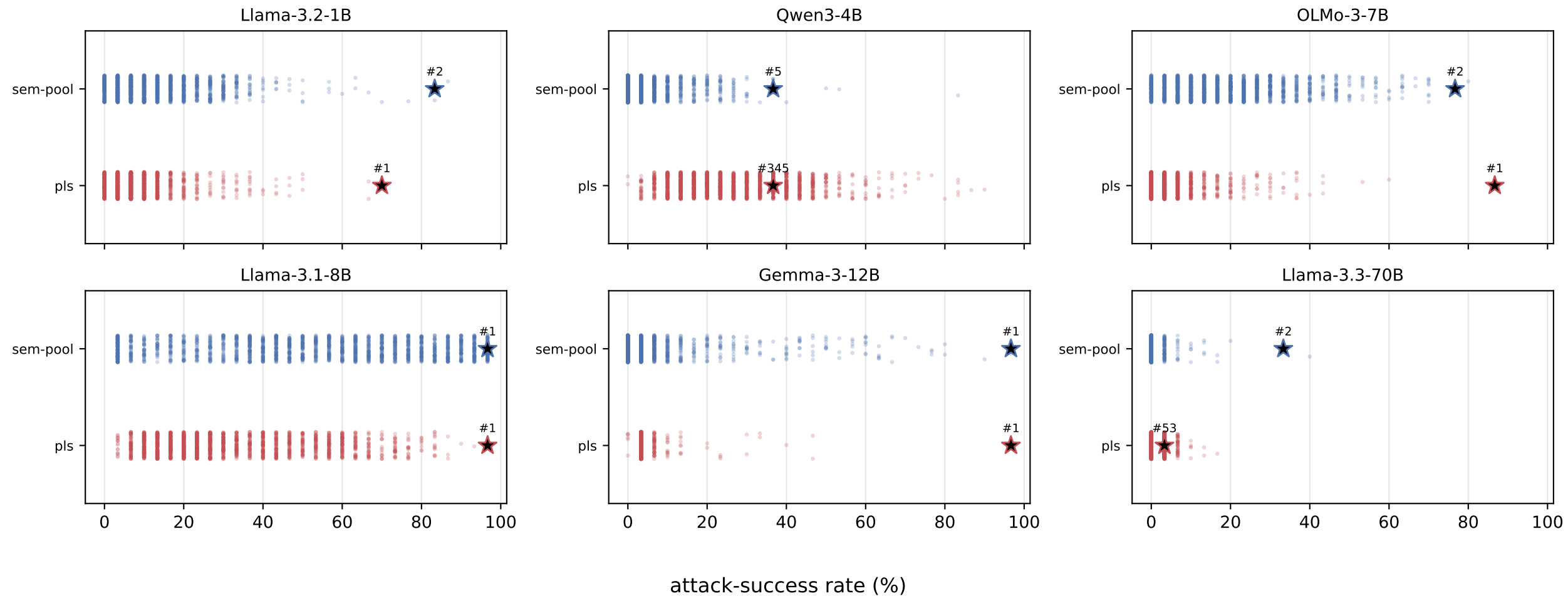
refusal: candidate ASR cloud (faded) vs planted trigger (★, with rank)
