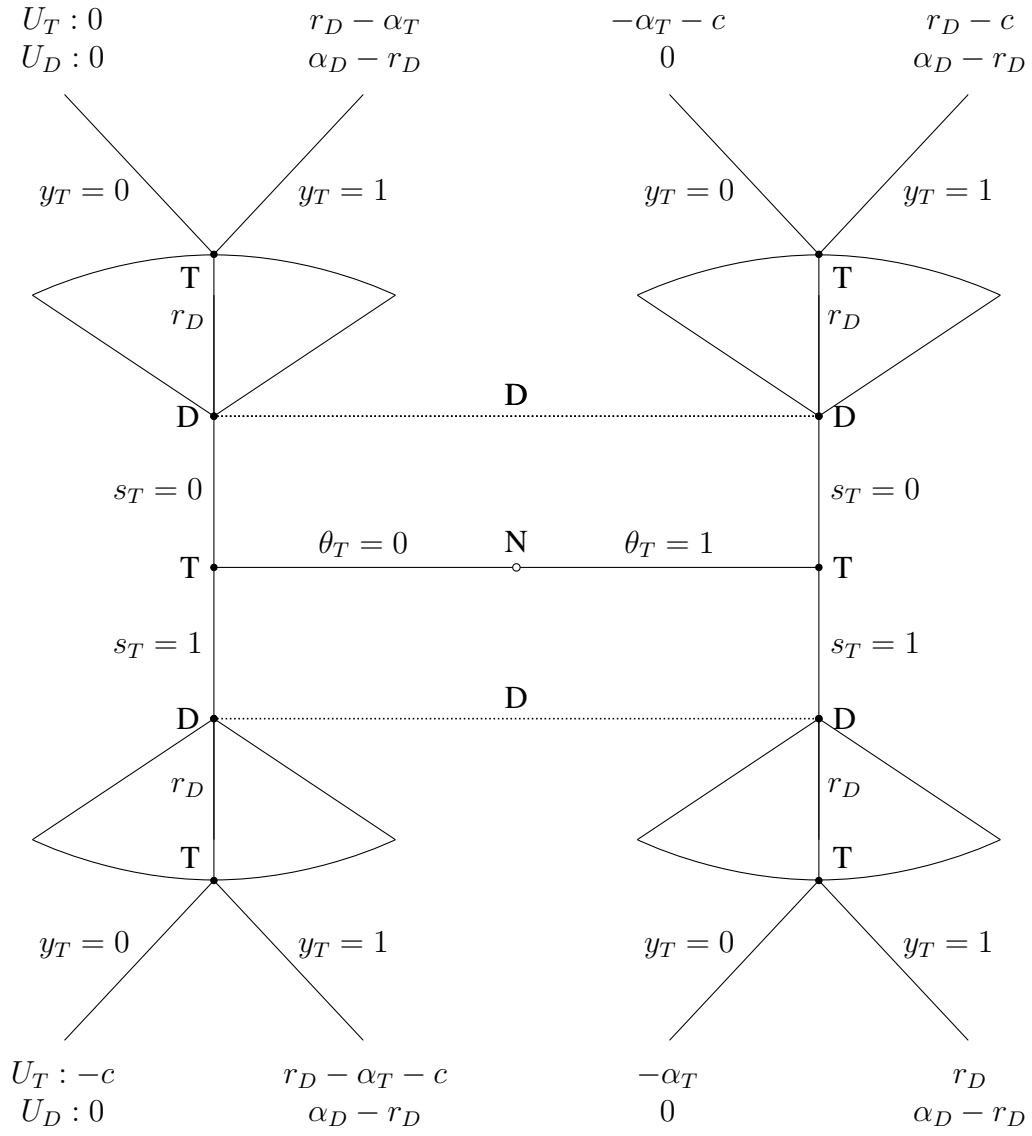
Figure 1: Game Tree
