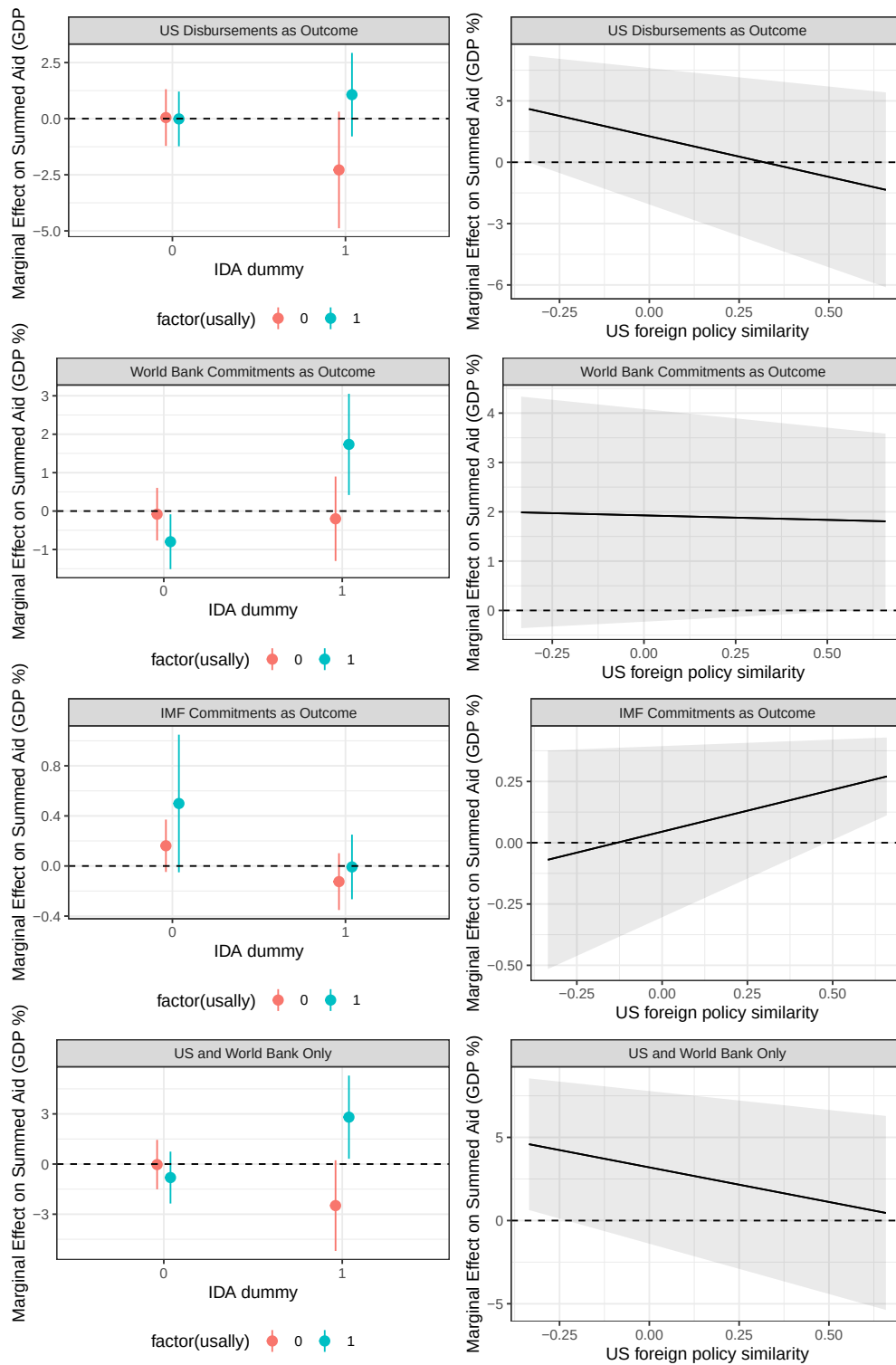
Figure 10: Marginal Effect of Strategic Nonresponse with Disaggregated Outcome.
