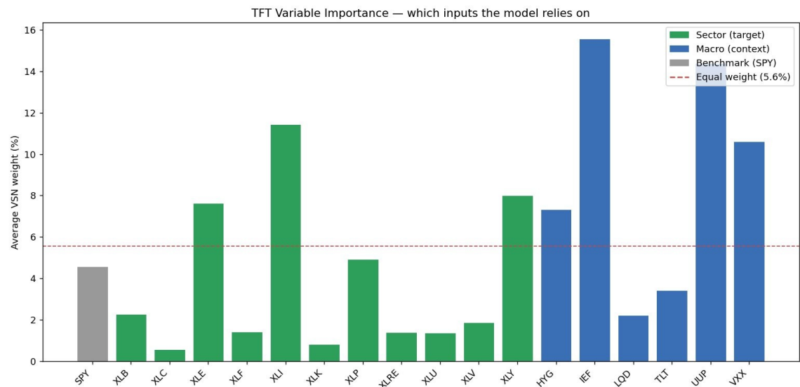
Figure: Average Variable Selection Network weight per input variate. Green bars are sector ETFs (prediction targets), blue bars are macroeconomic context variates, gray is the SPY benchmark. The dashed line marks equal weight (5.6%).
