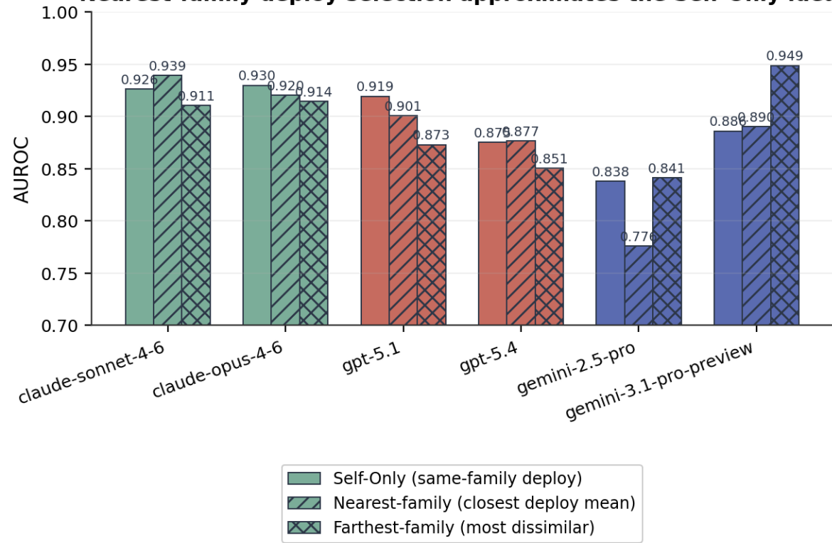
Nearest-family deploy selection approximates the Self-Only ideal
